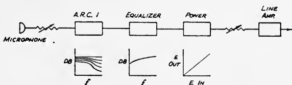
FIG. 9. Typical arrangement of amplifiers for sound recording.
